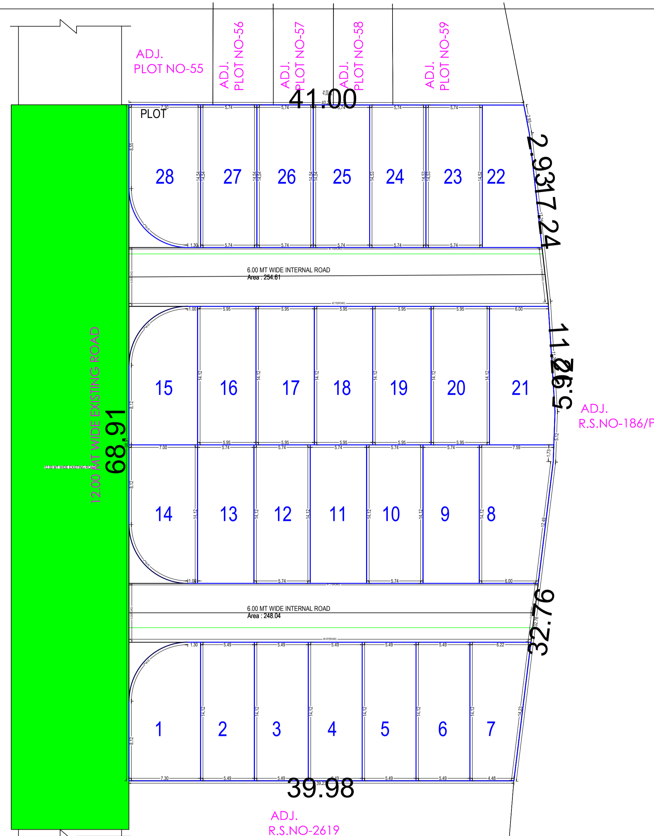
LAY OUT PLAN SITE PLAN (Scale - 1:400)
